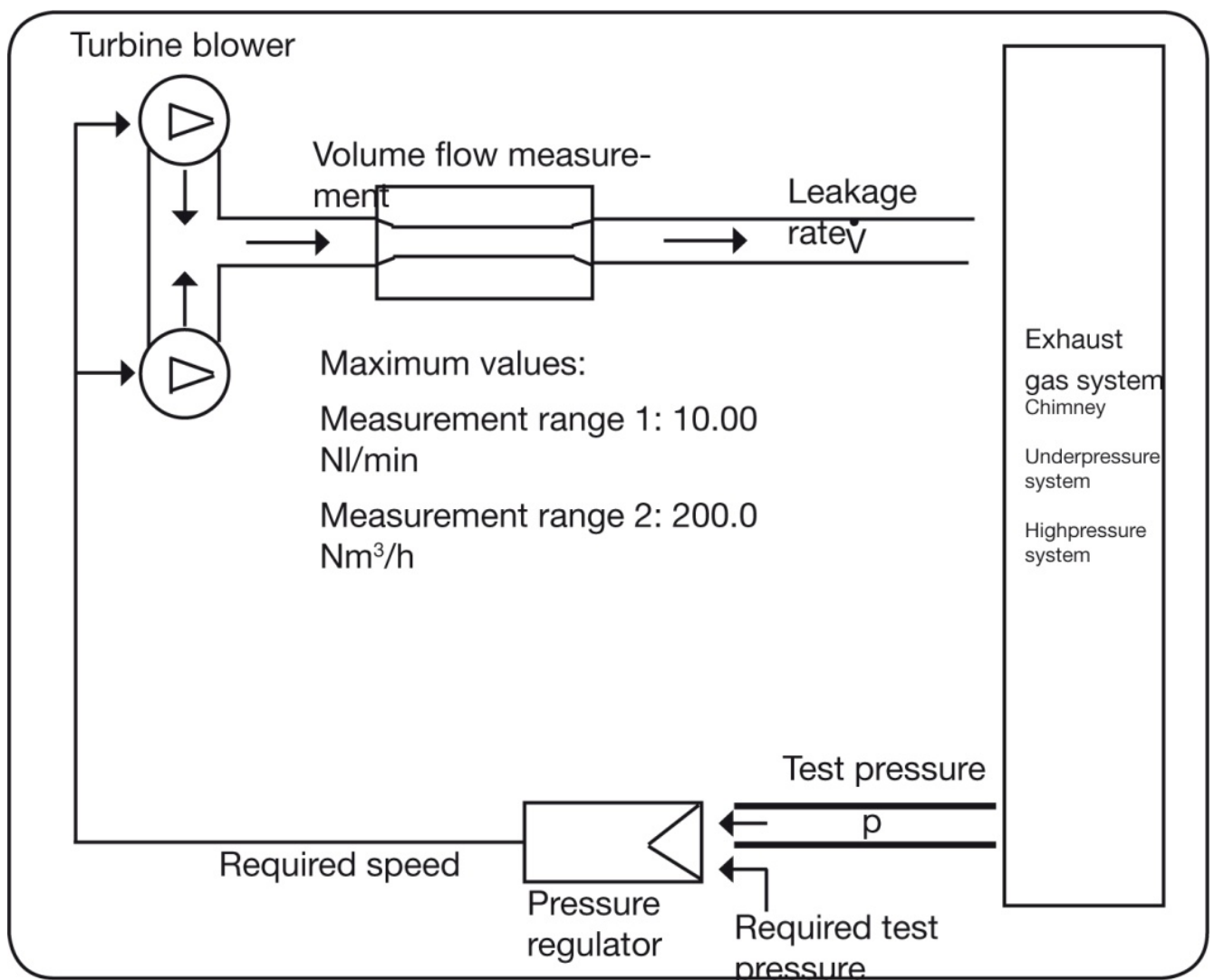
Fig. 7: Measuring principle Wöhler DP 600
