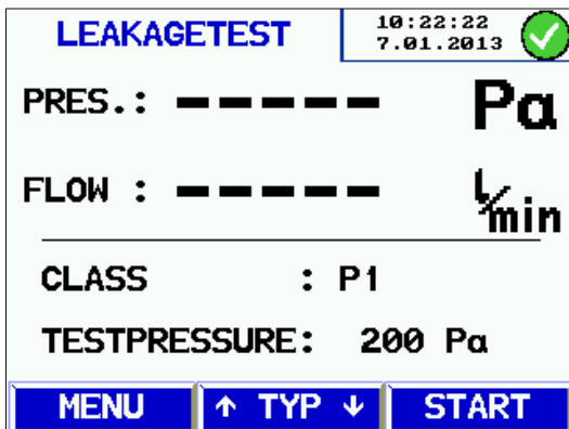
Fig. 22: Leakage test of an exhaust gas installation class P1
