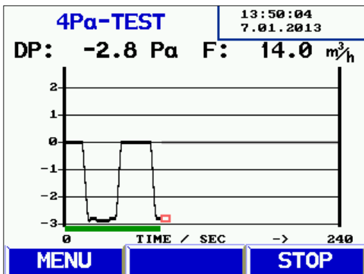
Fig. 40: Pressure profile during the 4 Pa Test
