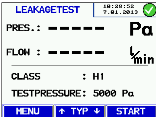
Fig. 23 Leakage test of an exhaust gas installation class H1
