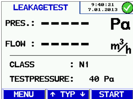
Fig. 21: Leakage test of exhaust gas installations class N1
