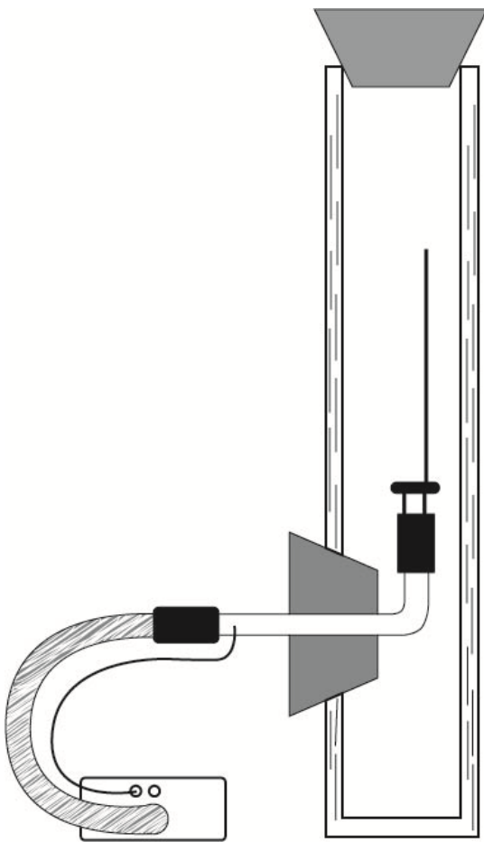
Fig. 20: Schematic drawing of a brick lined chimney
