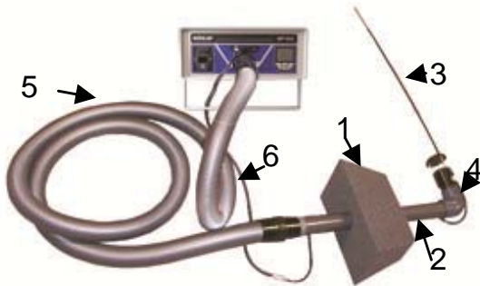
Fig. 14: Assembling the Probe Class N
